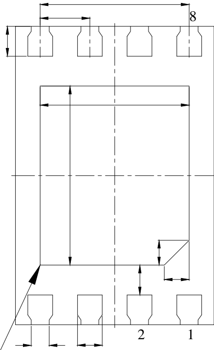
BOTTOM VIEW
