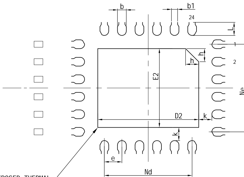
BOTTOM VIEW
