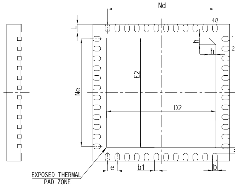
BOTTOM VIEW
